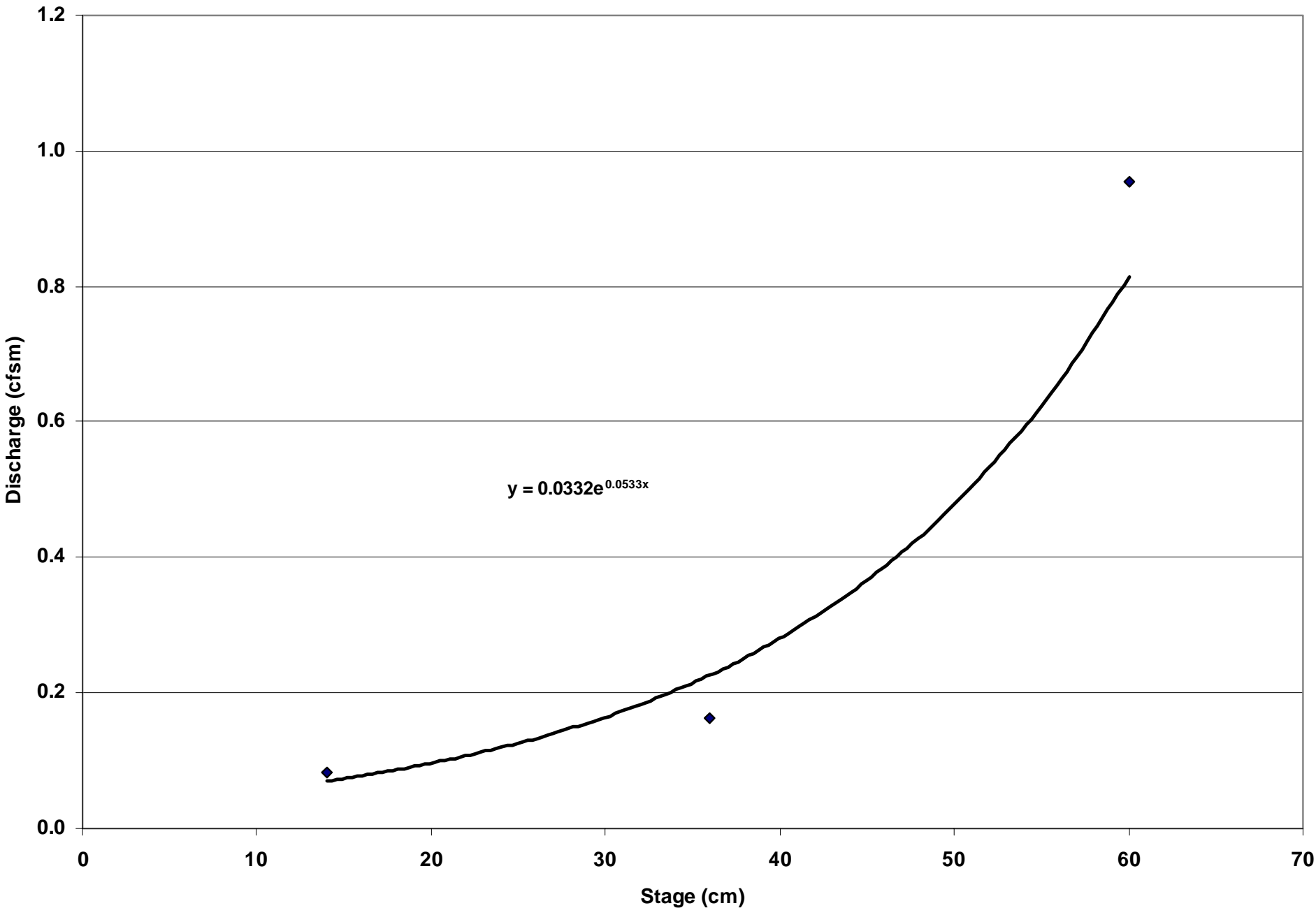
AI:6 Stage vs. Discharge for below Hatfield Dam
