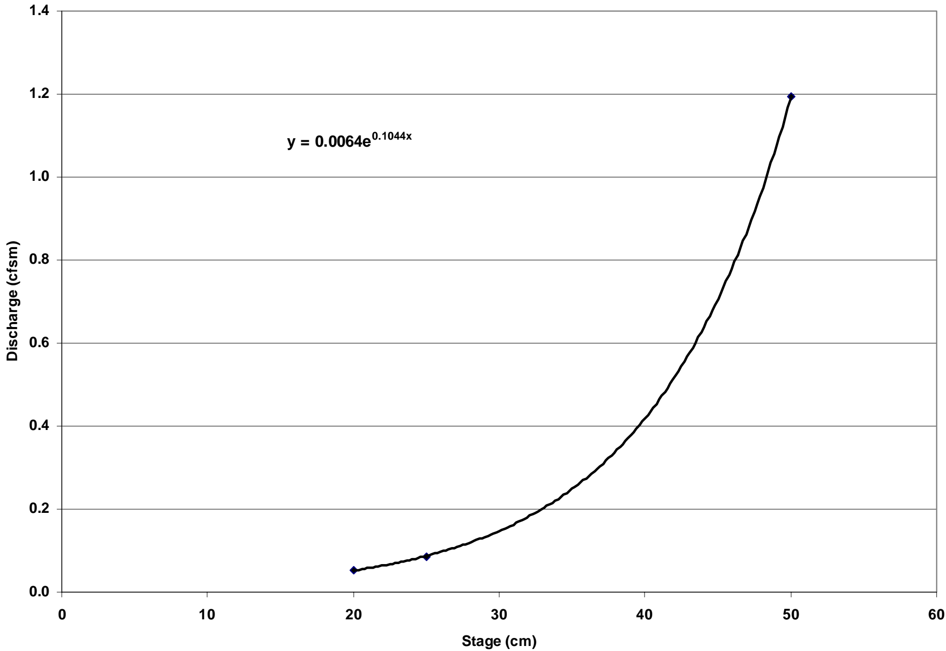
A1:5 Stage vs. Discharge for below West Brook
