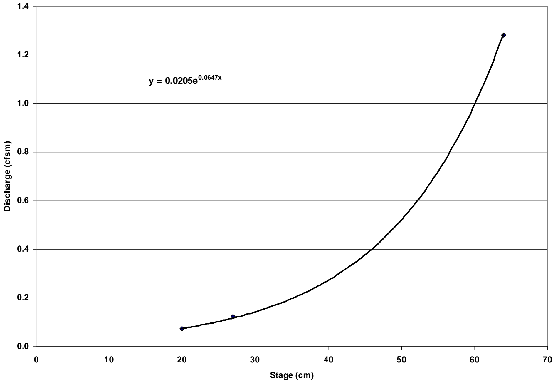
AI:4 Stage vs. discharge for above West Brook gage
