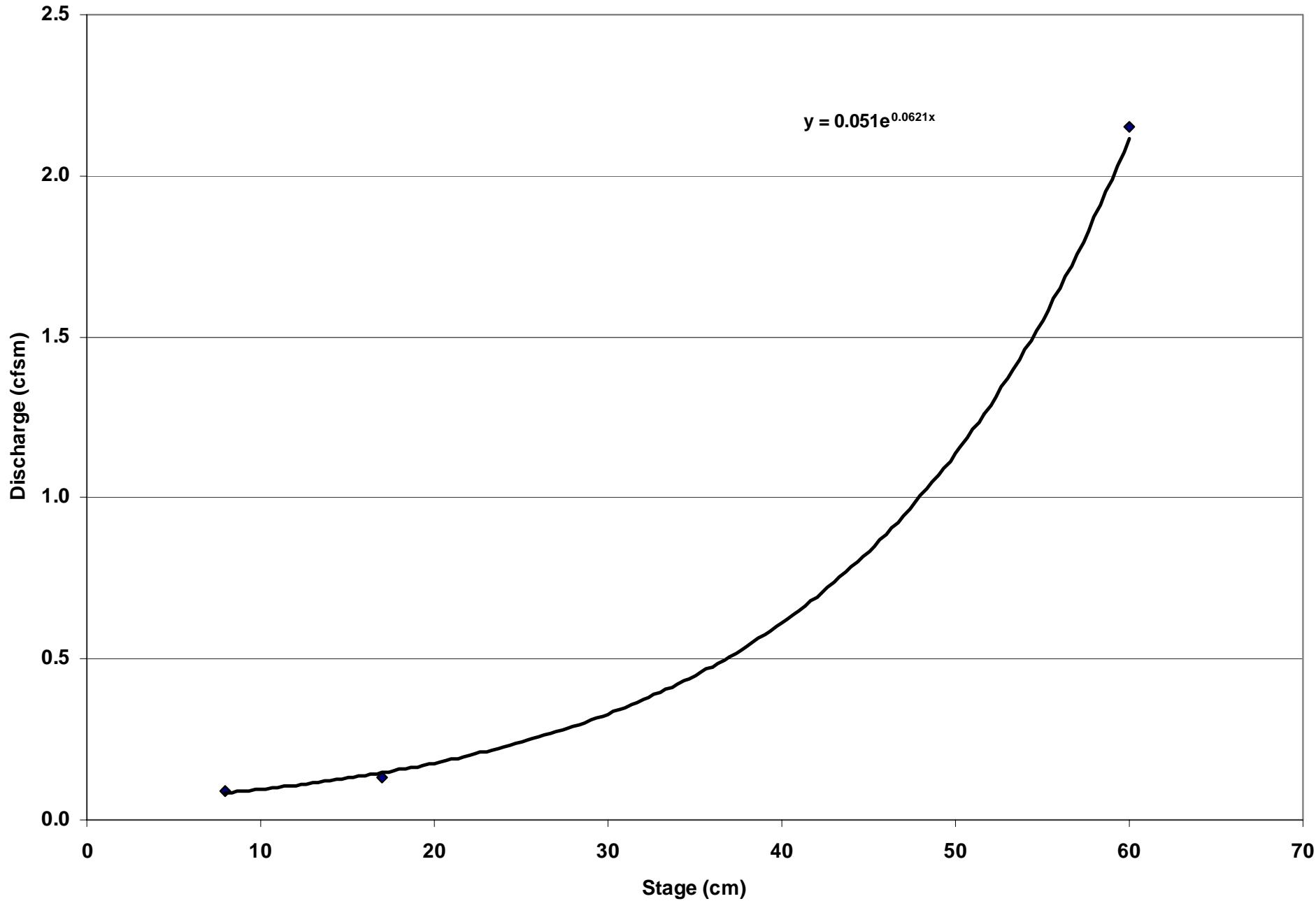
A1:1 Stage vs. discharge for below Esther Brook gage
