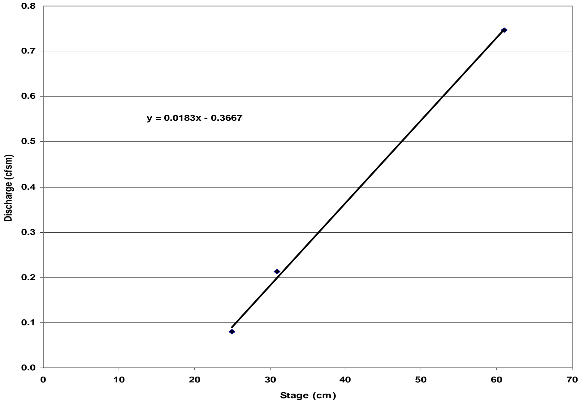
AI:2 Stage vs. discharge for Christian Lane gage
