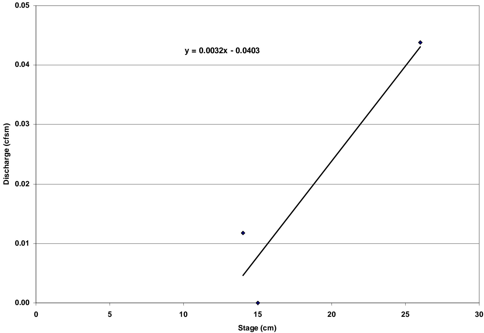
A1:3 Stage vs. discharge for Great Swamp Brook gage
